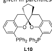
L10
