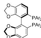
L11: (R)-DTBM-segphos
